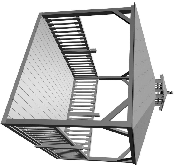
Lindrick Canopy with floor and balustrade NR. ART. C42103
